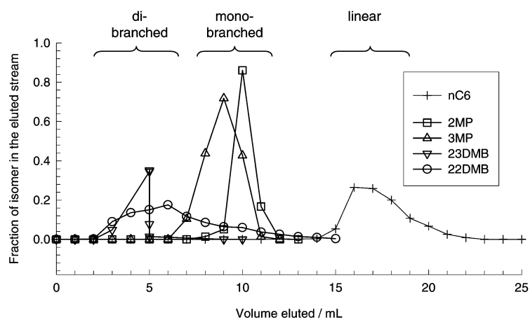
Fig. 14 (a) CBMC simulations of component loadings for equimolar mixture of nC_6 , 2MP, 3MP, 22DMB and 23DMB in MFI at 300 K. (b) Elution profiles in a pulsed chromatographic experiment. 40
